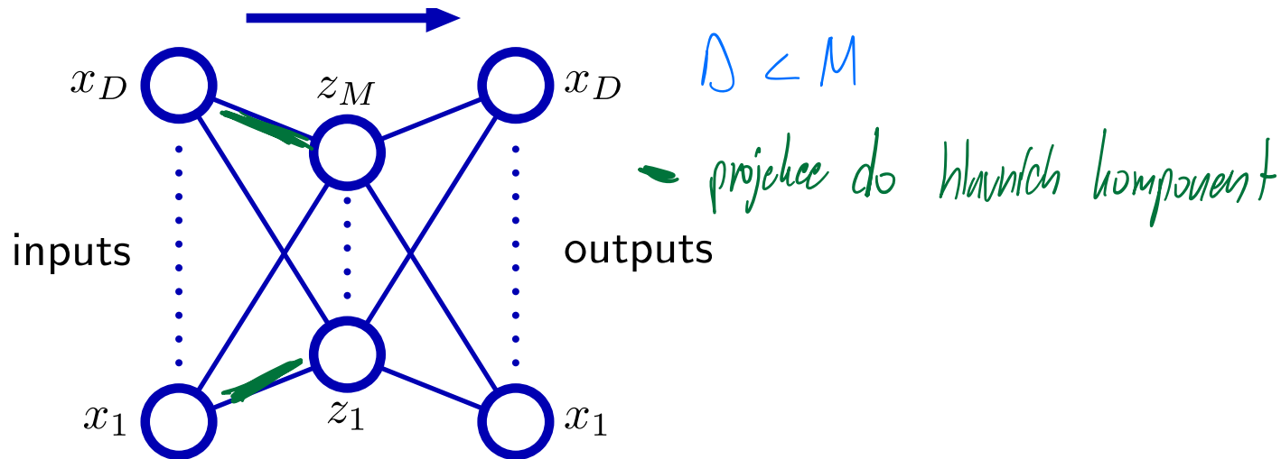
Figure 12.8 of Pattern Recognition and Machine Learning.
