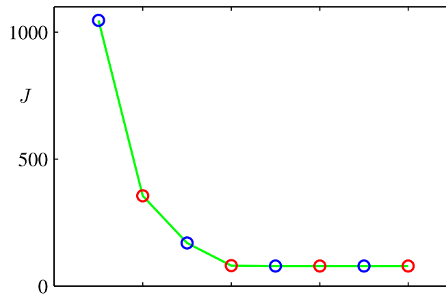
Figure 9.2 of Pattern Recognition and Machine Learning.
