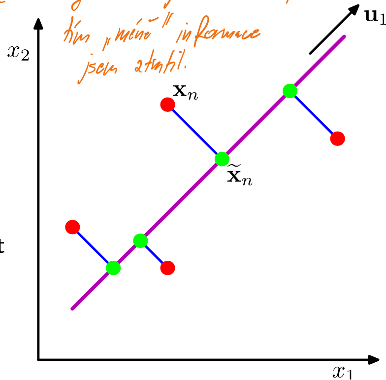
Figure 12.2 of Pattern Recognition and Machine Learning.
