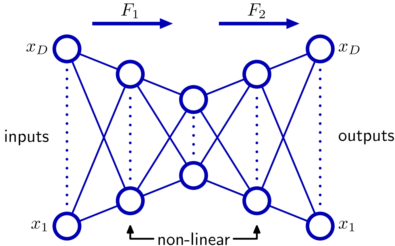
Figure 12.9 of Pattern Recognition and Machine Learning.
