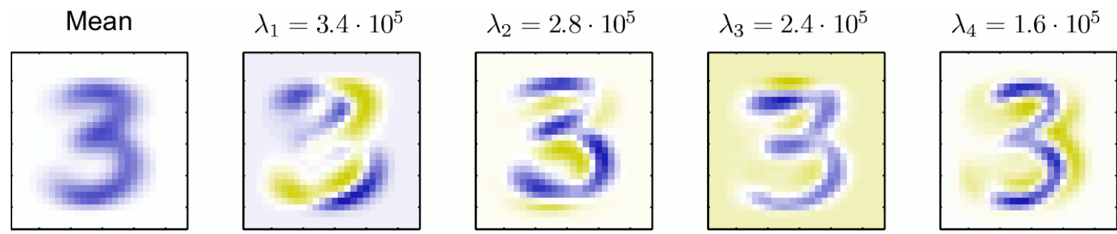
Figure 12.3 of Pattern Recognition and Machine Learning.
