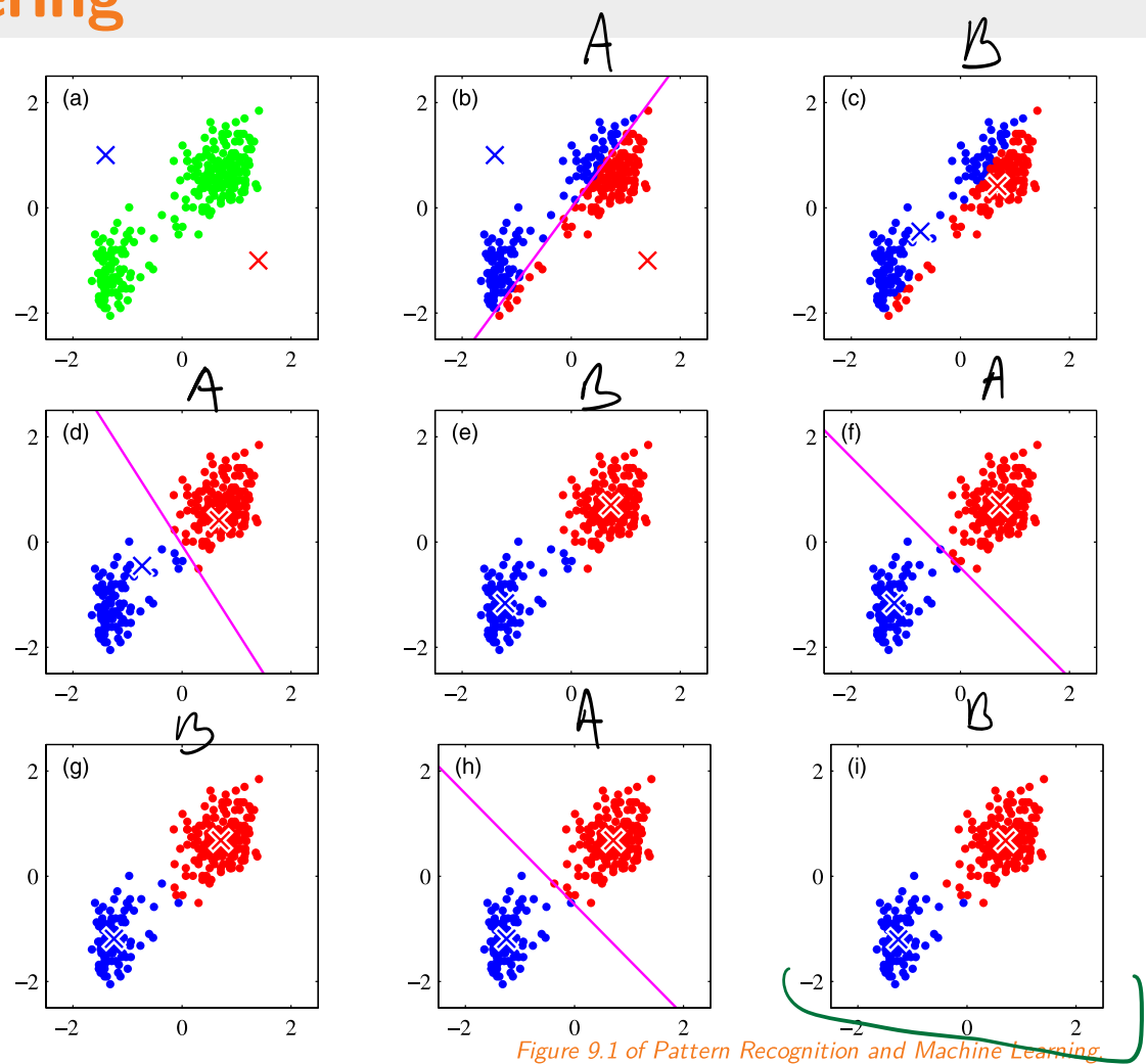
Figure 9.1 of Pattern Recognition and Machine Learning
